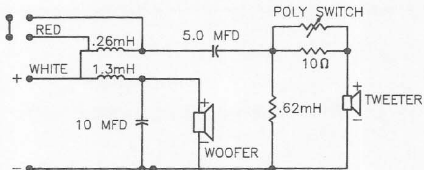
CROSSOVER SCHEMATIC
